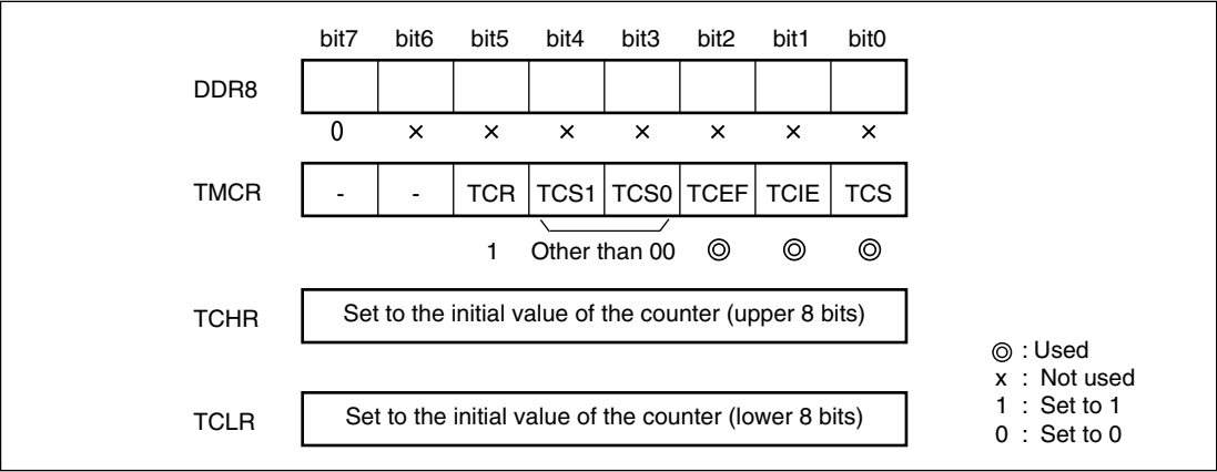
Figure 12.7-1 Setting the Counter Function
