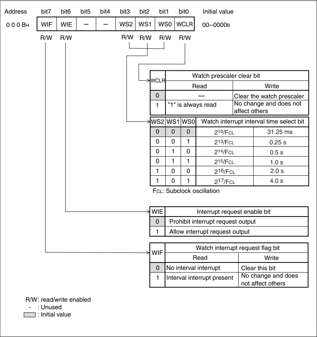
Figure 7.3-1 Watch Prescaler Control Register (WPCR)
