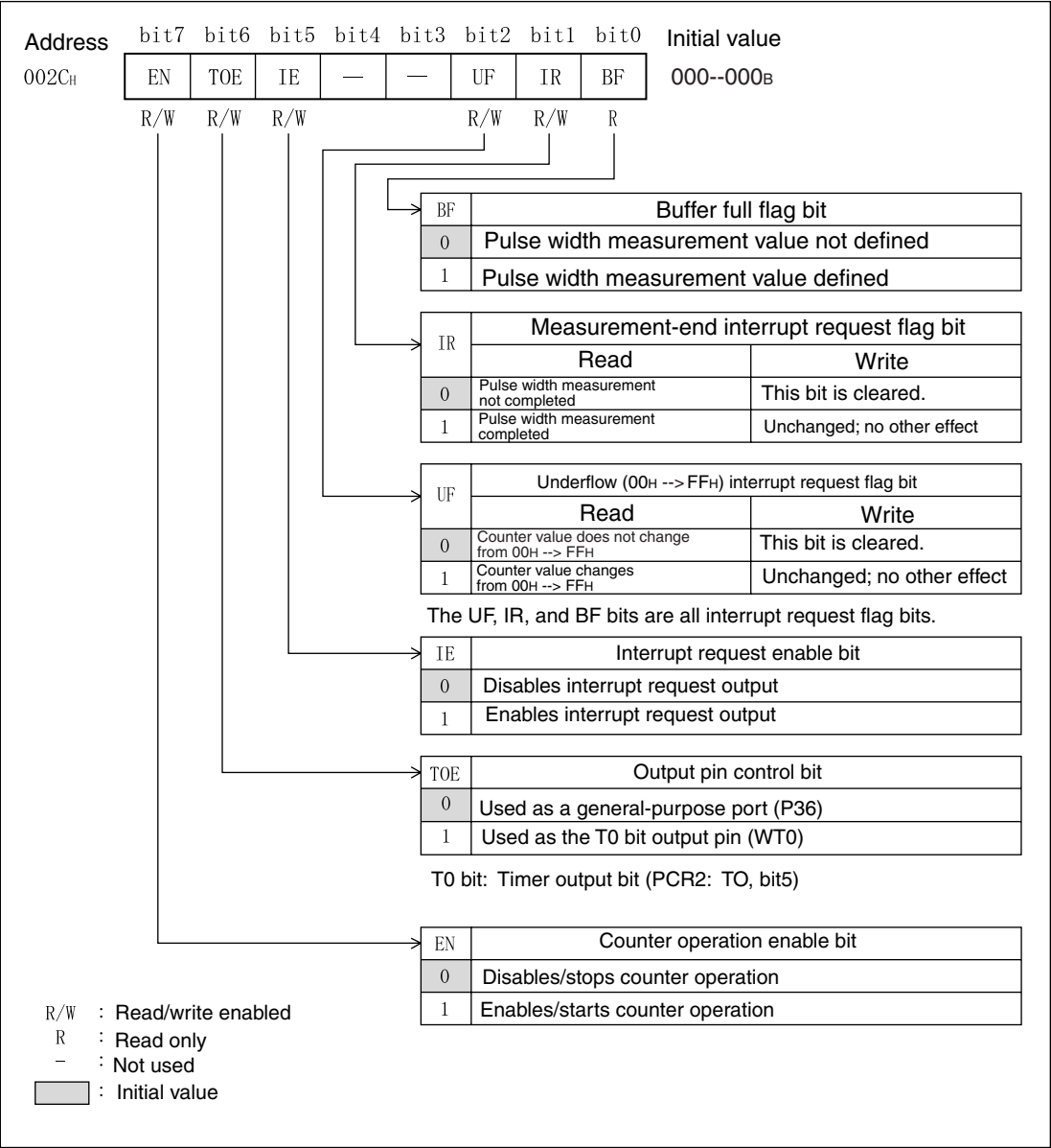
Figure 9.4-2 PWC Pulse Width Control Register 1 (PCR1)
