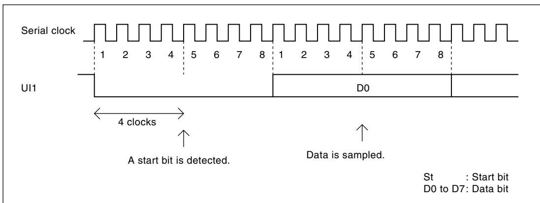
Figure 16.7-6 Detecting a Start Bit
