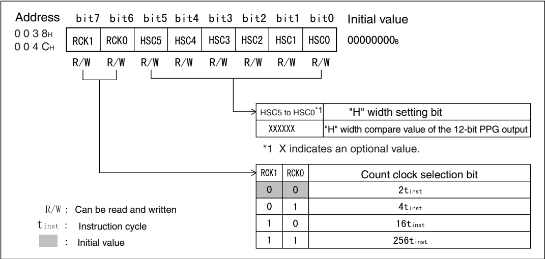
Figure 11.4-2 12-bit PPG Control Register 1 (PPGC1/PPGC2)
