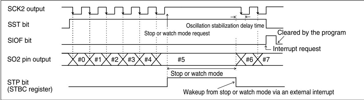
Figure 18.8-2 Operation in Stop or Watch Mode (Internal Shift Clock)
