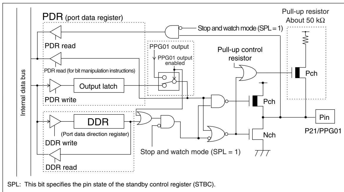
Figure 11.3-1 Block Diagram of the P21/PPG01 Pins
