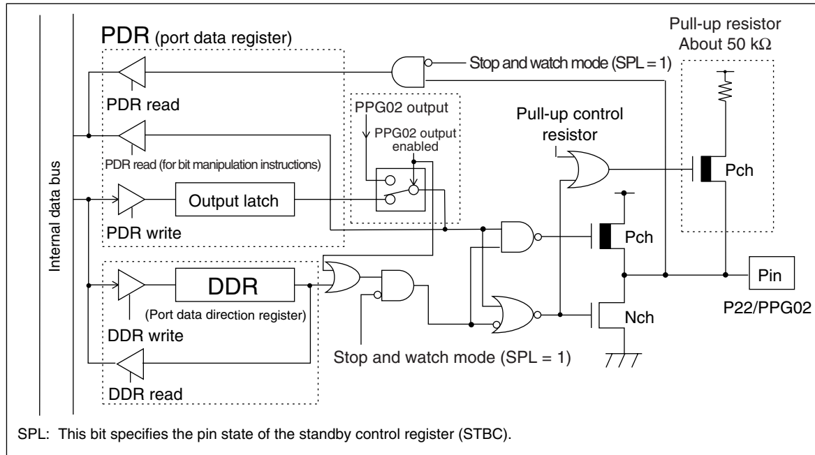
Figure 11.3-2 Block Diagram of P22/PPG02 Pin
