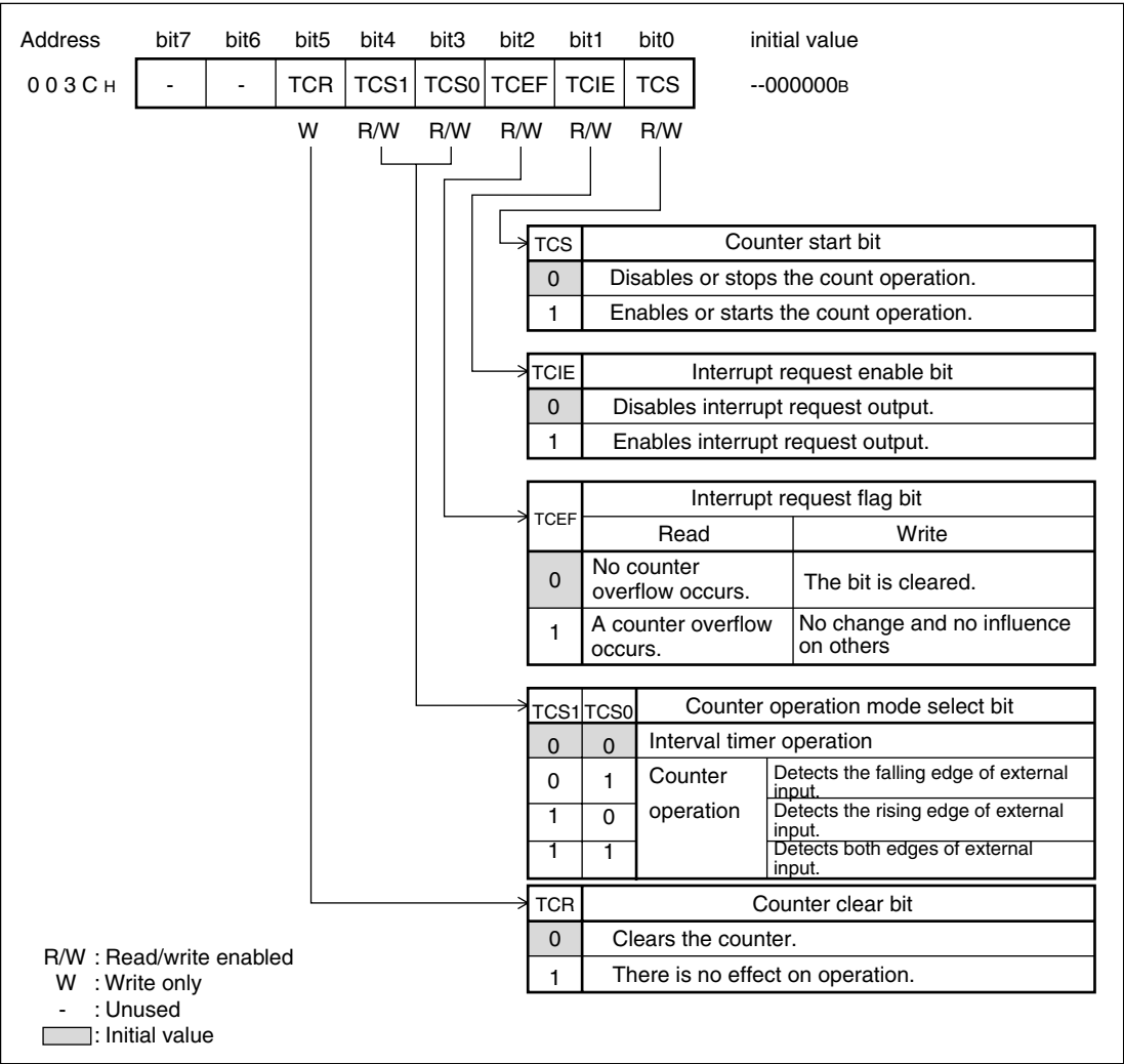
Figure 12.4-2 Timer Control Register (TMCR)
