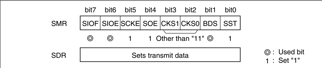
Figure 18.6-1 Serial Output Settings (for an Internal Shift Clock)
